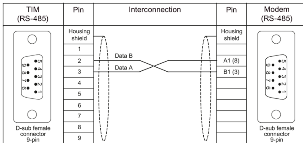
Figure A-7 Assignment of the cable for the RS-485 interface
