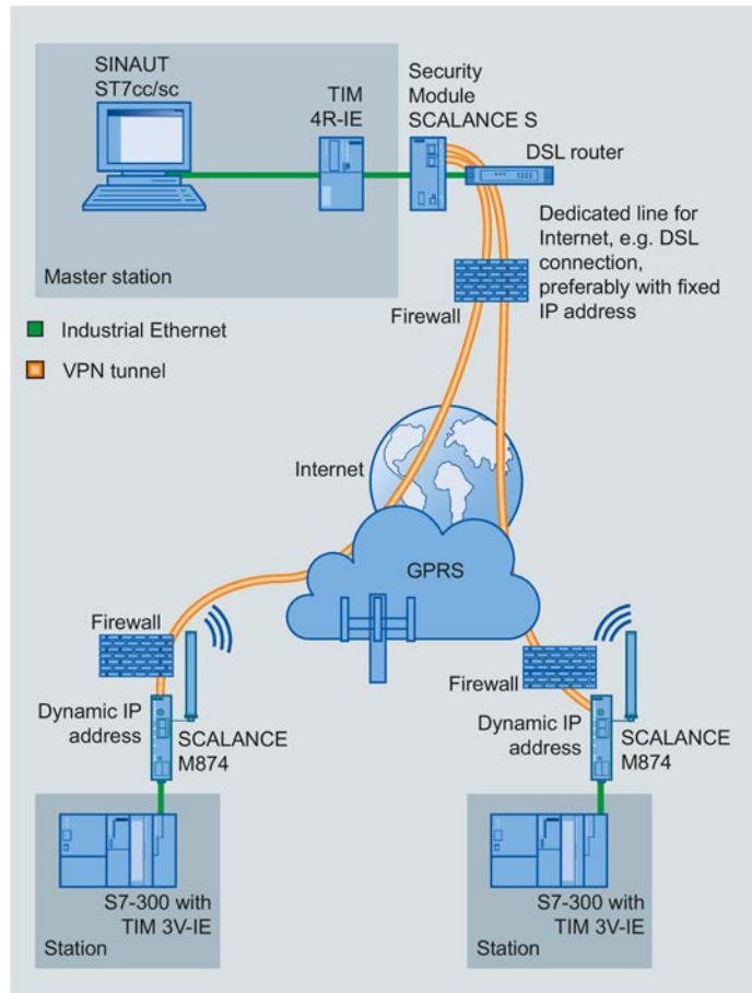
Figure 3-6 GPRS with higher security via SCALANCE M874 router
