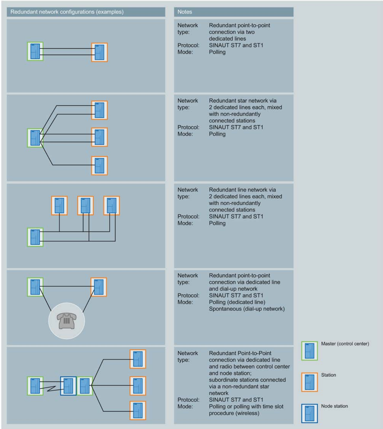
Figure 3-10 Redundant configurations
