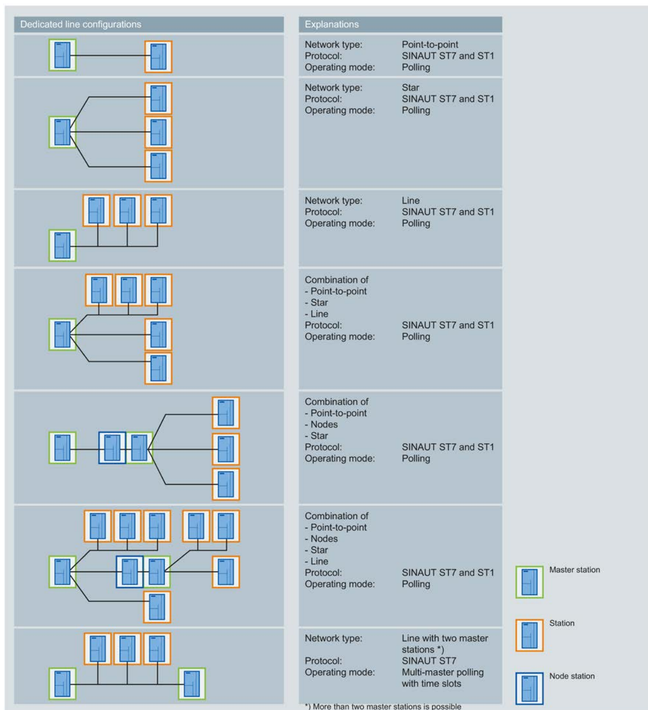
Figure 3-7 Dedicated line configurations
